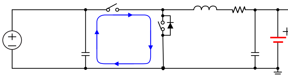
Figure 37. High Frequency Current Path
