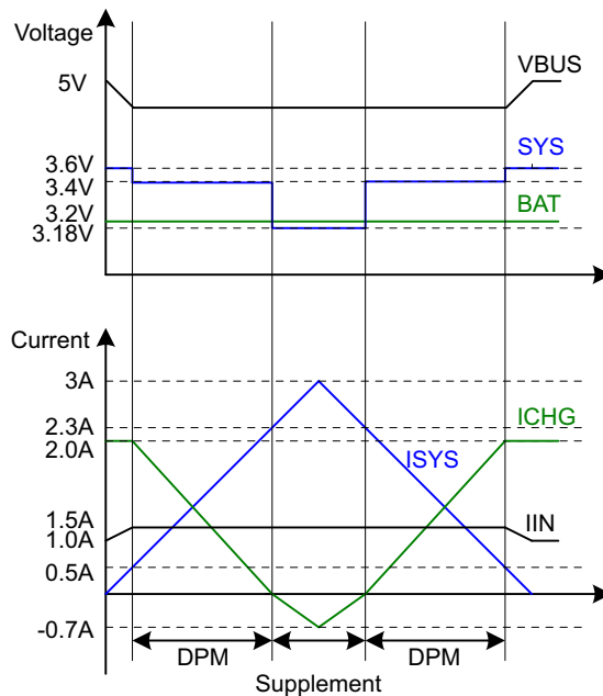
Figure 25. DPM Response
