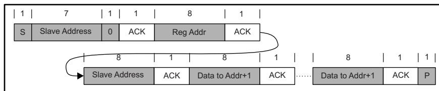
Figure 38. Multi-Write
