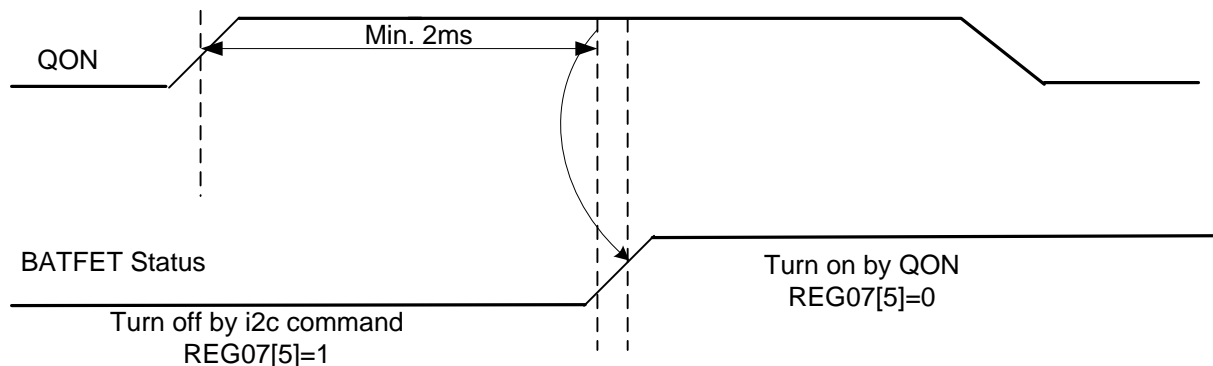
Figure 22. QON Timing
