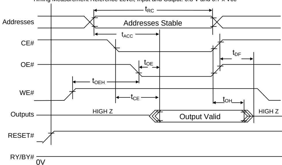
Figure 5. AC Waveforms for READ Operations
