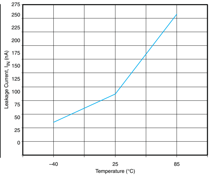
Figure 7. I_{IN} Leakage Current vs. Temperature ( V_{IN} = 3.3\text{ V} )
