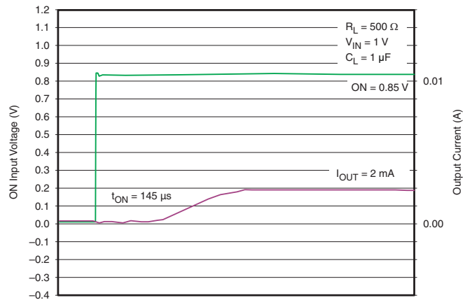
Figure 21. t_{ON} Response
