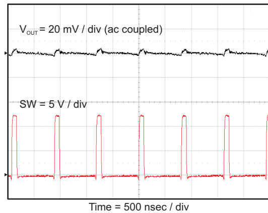
Figure 33. Output Voltage Ripple, I_{OUT} = 10 \text{ mA}
