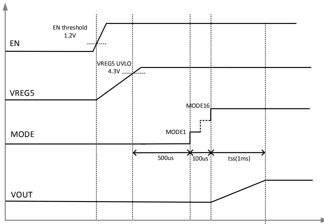
Figure 21. Power-Up Sequence
