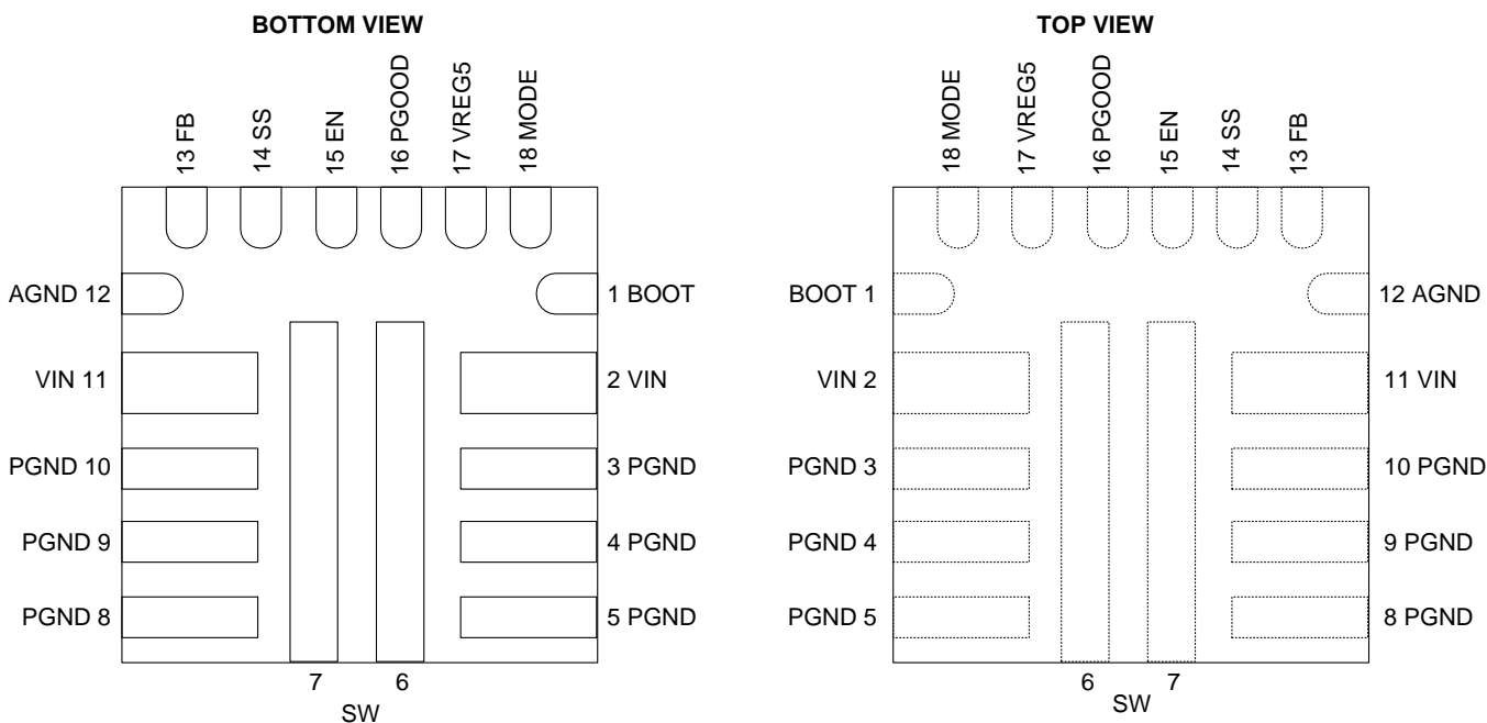
Pin Functions
