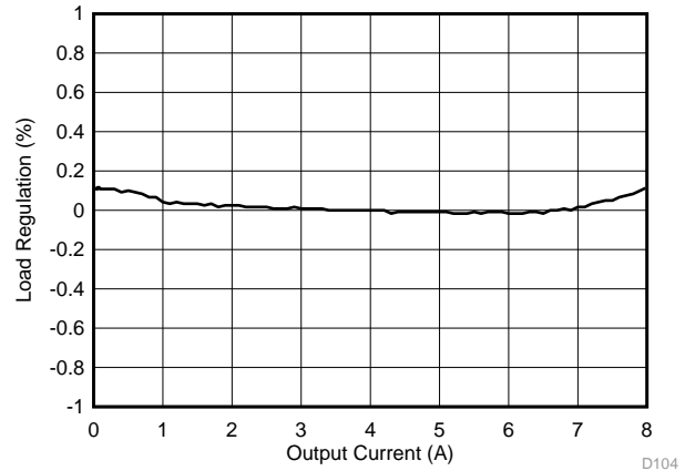
Figure 27. Load Regulation, V_{IN} = 12\text{ V}
