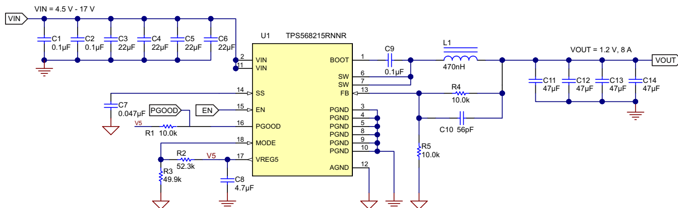
Figure 23. Application Schematic
