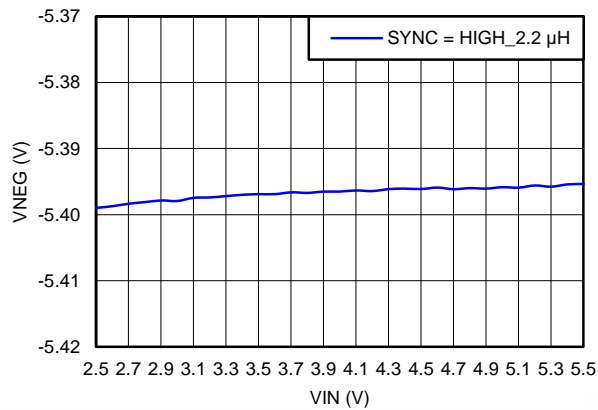
Figure 115. Line Regulation V NEG = -5.4 V — SYNC = HIGH
