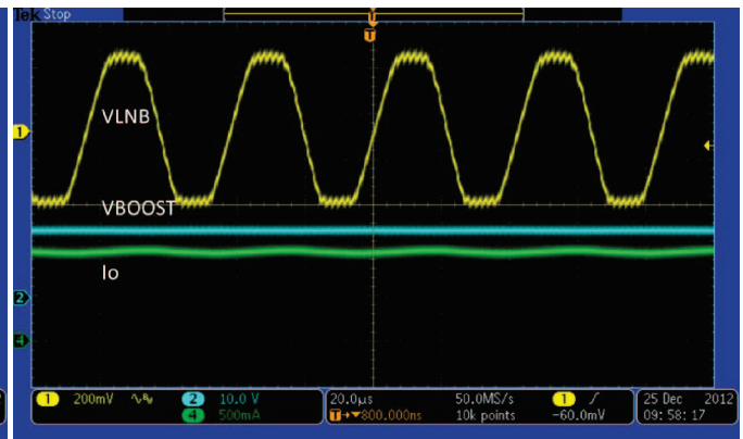
Figure 32. V_{IN} = 5\text{ V} , V_{LNB} = 13.4\text{ V} , 0.5 A, 22-kHz Tone
