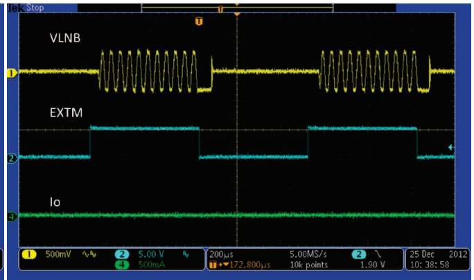
Figure 44. V_{IN} = 12\text{ V} , V_{LNB} = 13.4\text{ V} , No Loading, EXT_M Level
